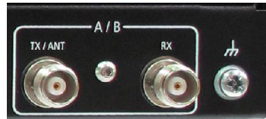
Rack mounted Aprisa SR+ Protected Station with duplexer
